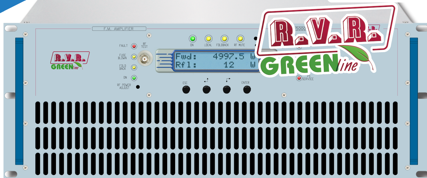
PJ5000U-K front view
